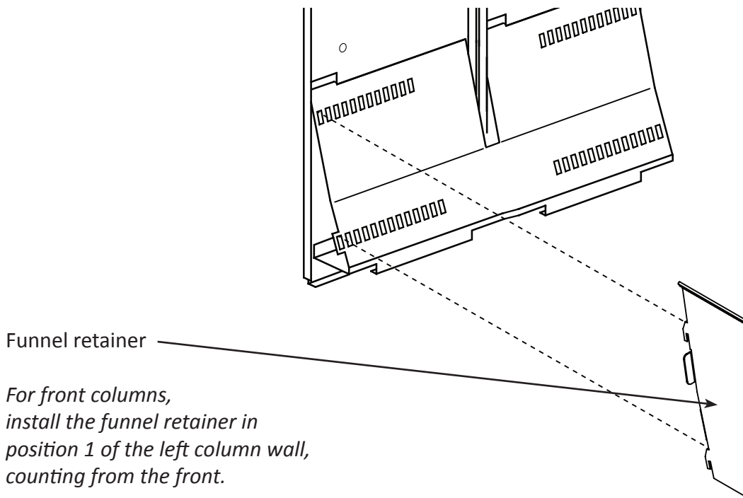
Figure 2. Funnel retainer installation.
