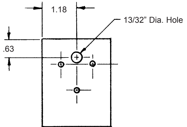
REAR VIEW OF OPENER
