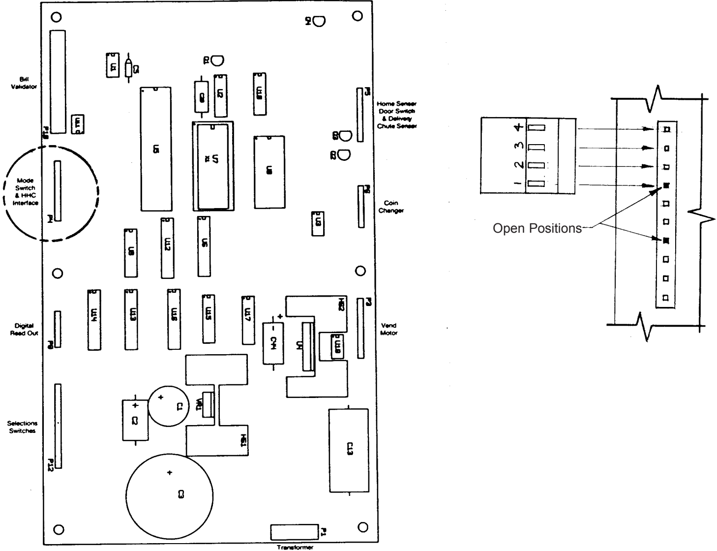
Controller Board Connector Layout
