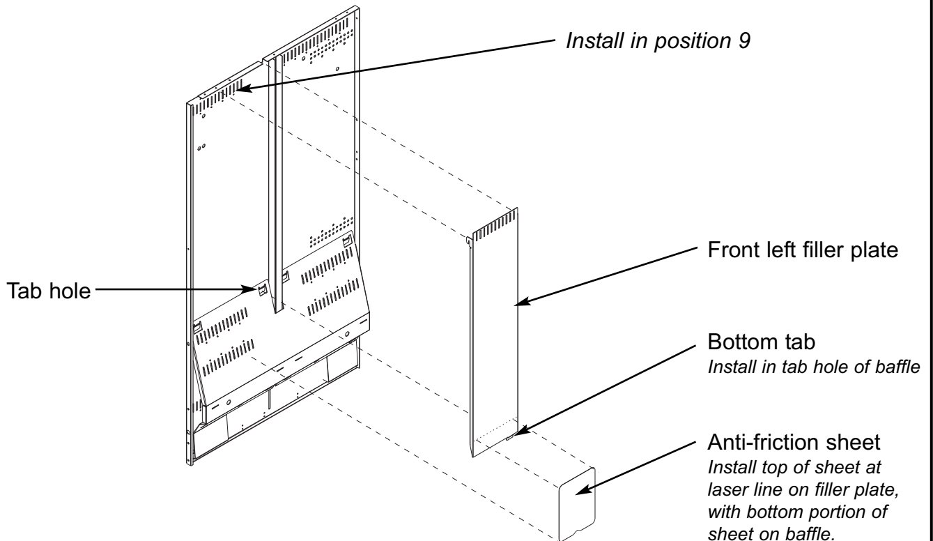
Figure 4 Installation of front filler plate - left column wall
