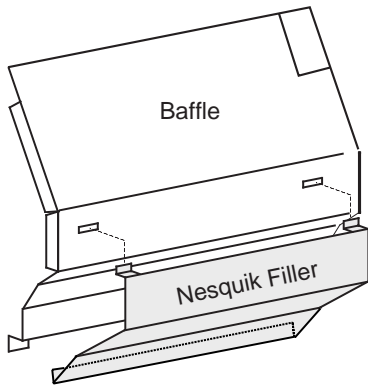
Figure 1 Installation of filler plate
